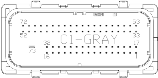
AEM Infinity Connectors Viewed from Wire Side
