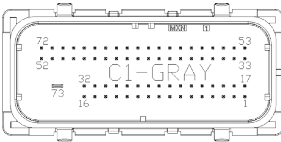
AEM Infinity Connectors Viewed from Wire Side
